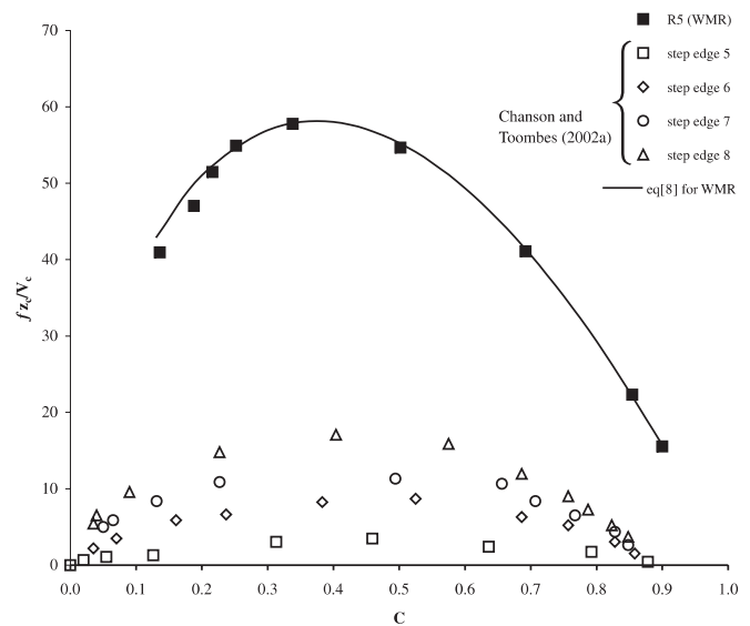
Fig. 10. Comparison of fz_c/V_c versus C data with the data of Chanson and Toombes (2002a) for WMR step configuration and q = 0.15 \text{ m}^2/\text{s} .
